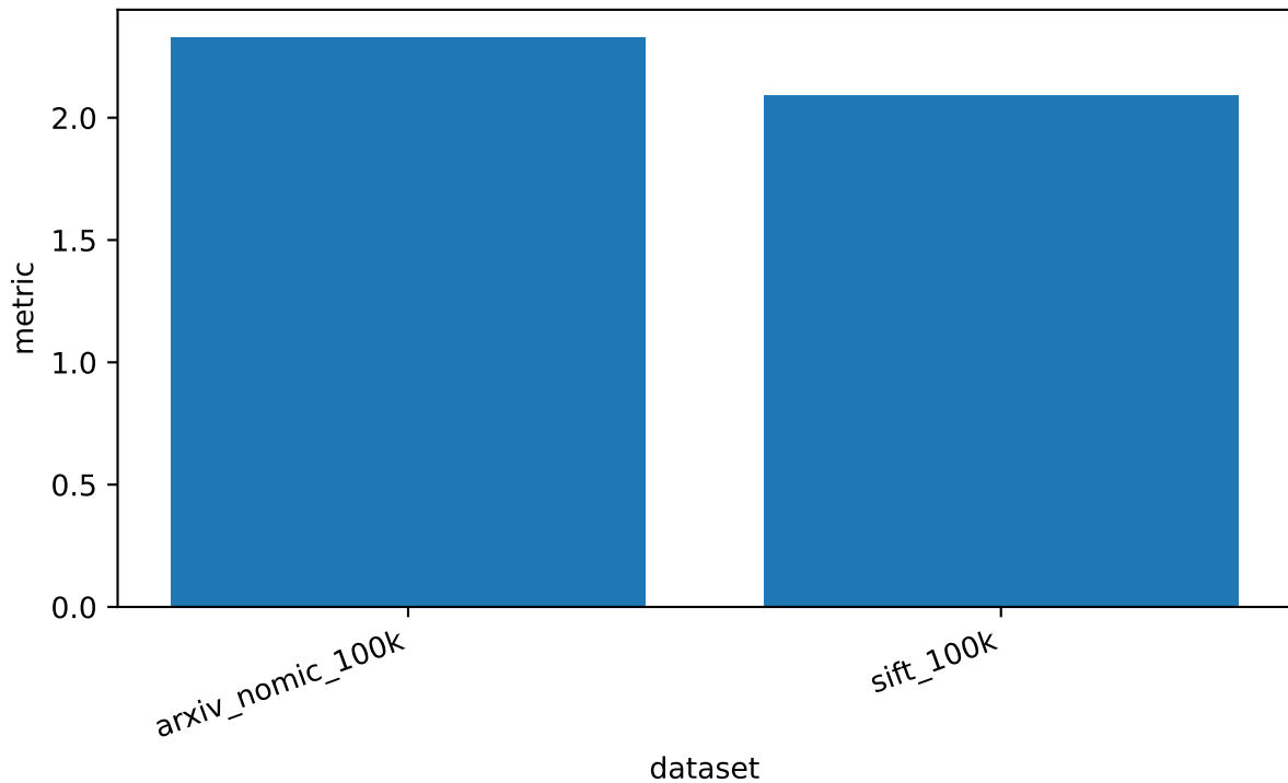
oracle entropy
