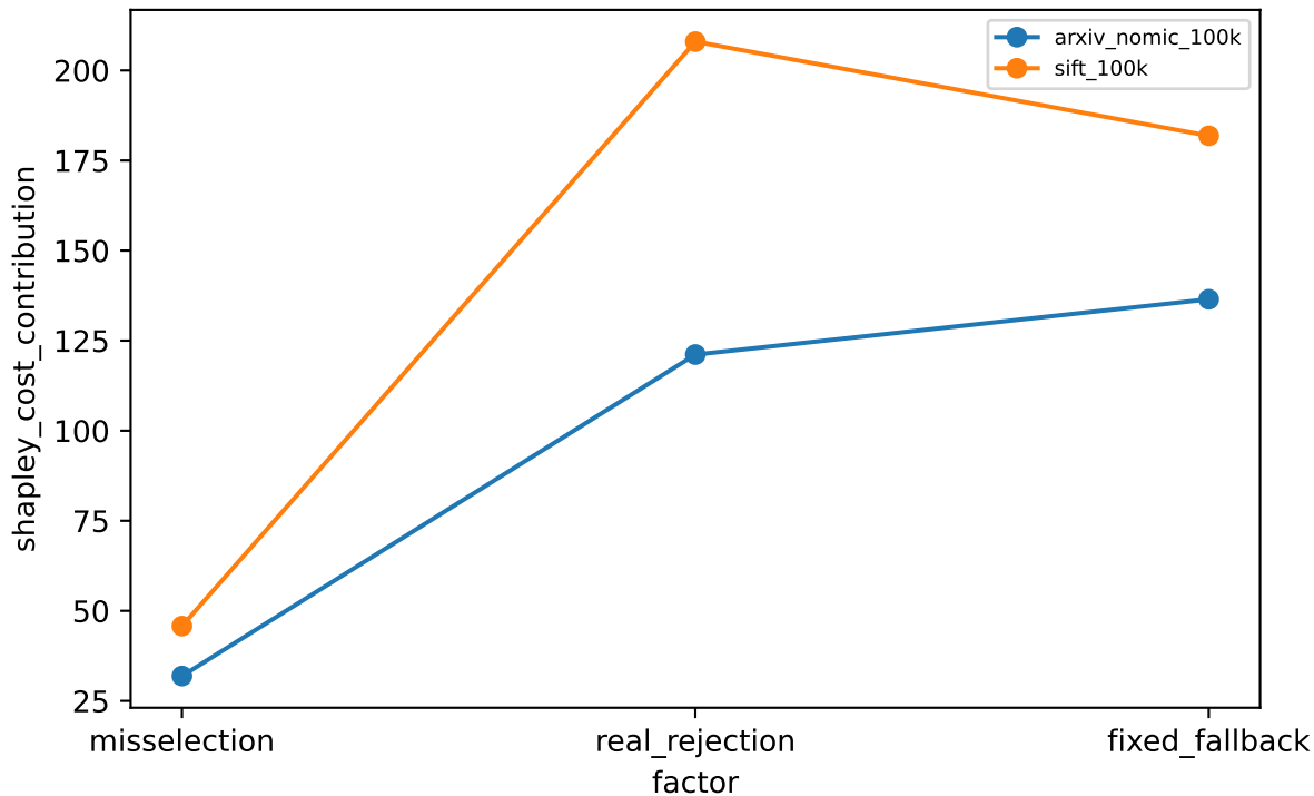
shapley mean
