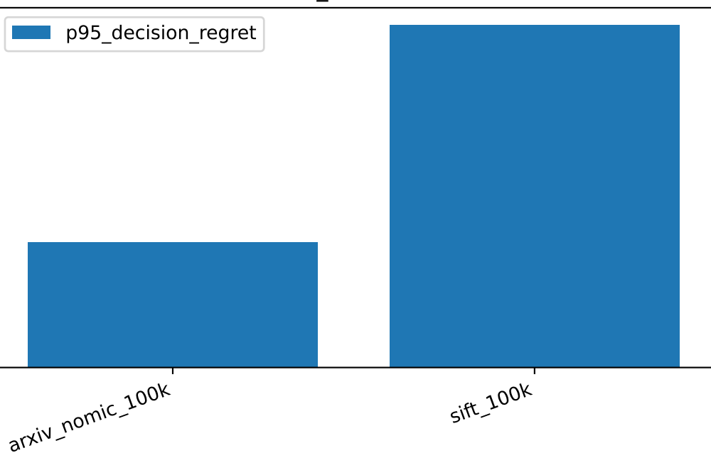
cost_confusion
