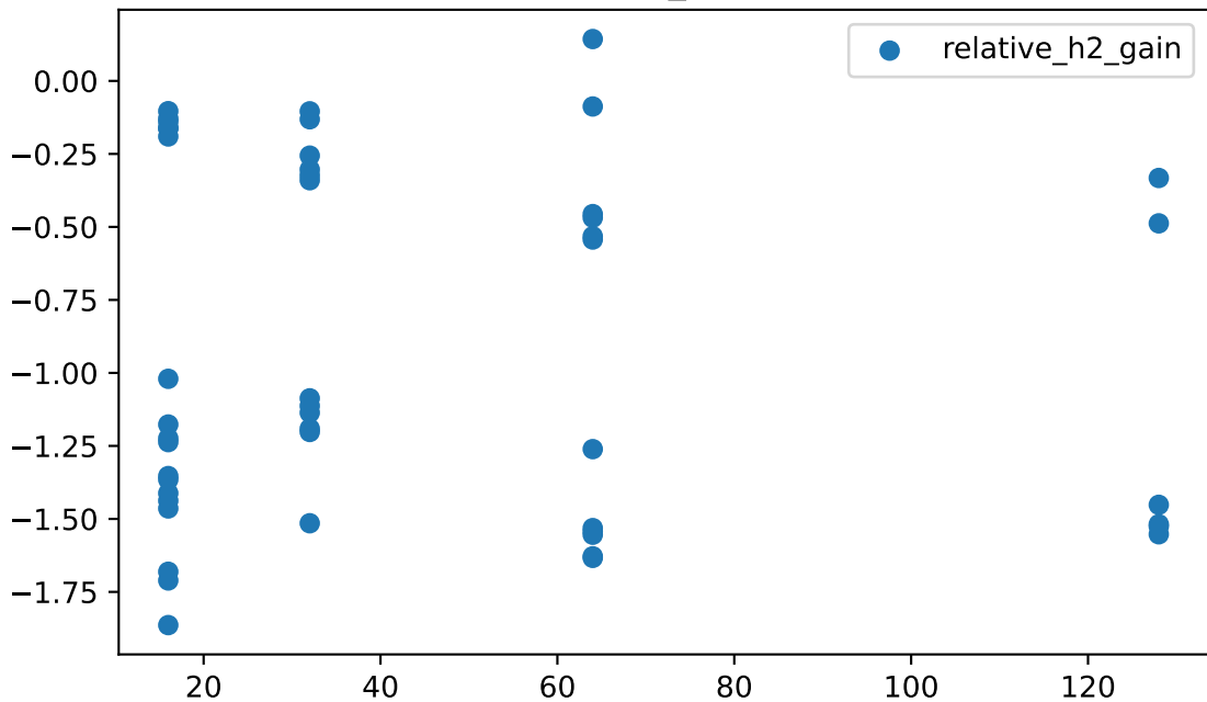
labels_gain
