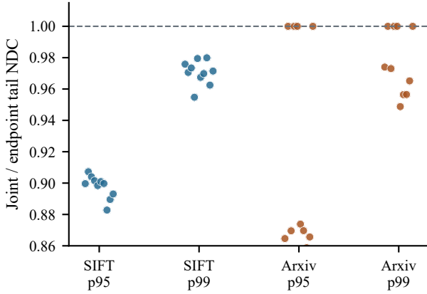
Figure 5: Per-target tail ratios for joint-error replay, relative to that target’s endpoint; ten dots per dataset/quantile. Equality reflects an endpoint fallback. All ratios are at most one. These descriptive tail comparisons are not formal non-inferiority certificates or wall-clock results.
