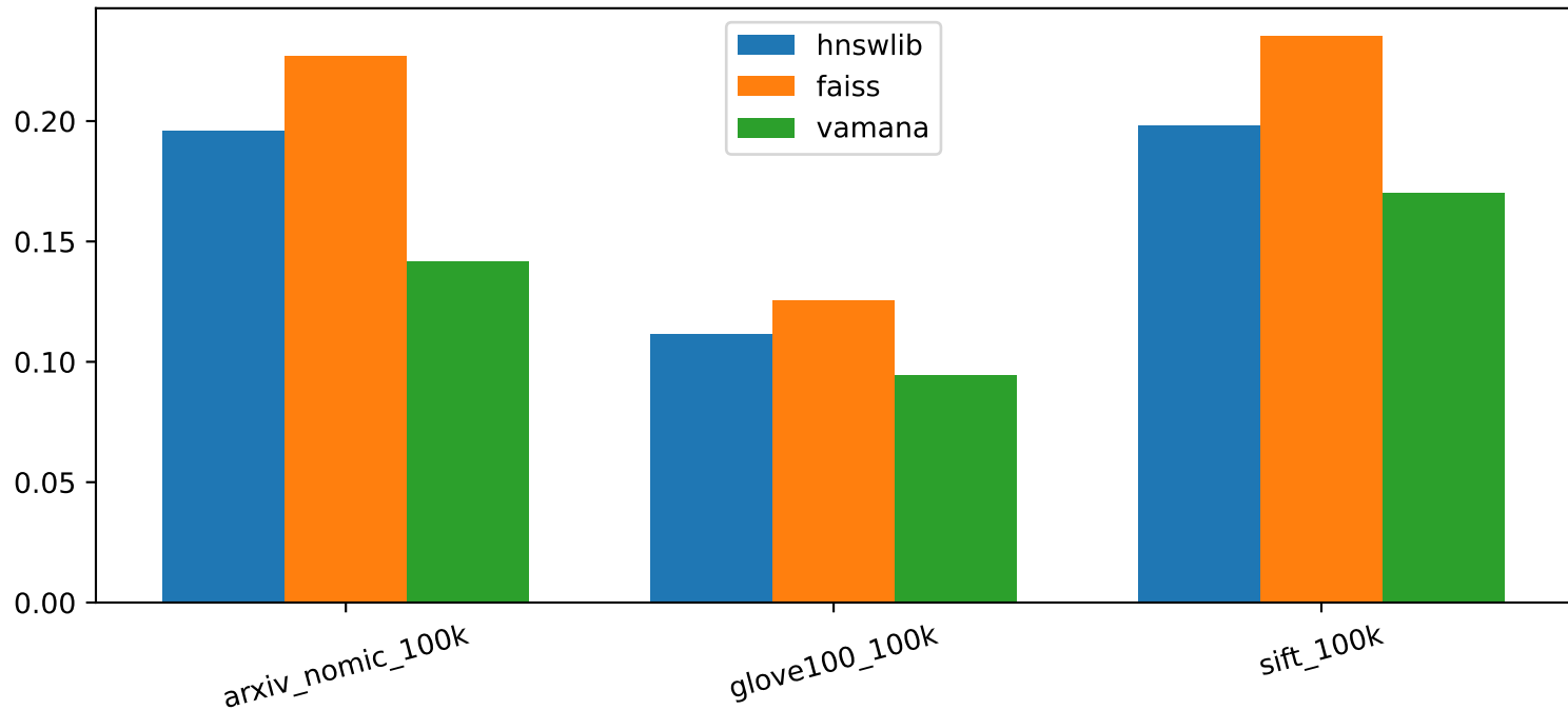
Mean pairwise rank inversion
