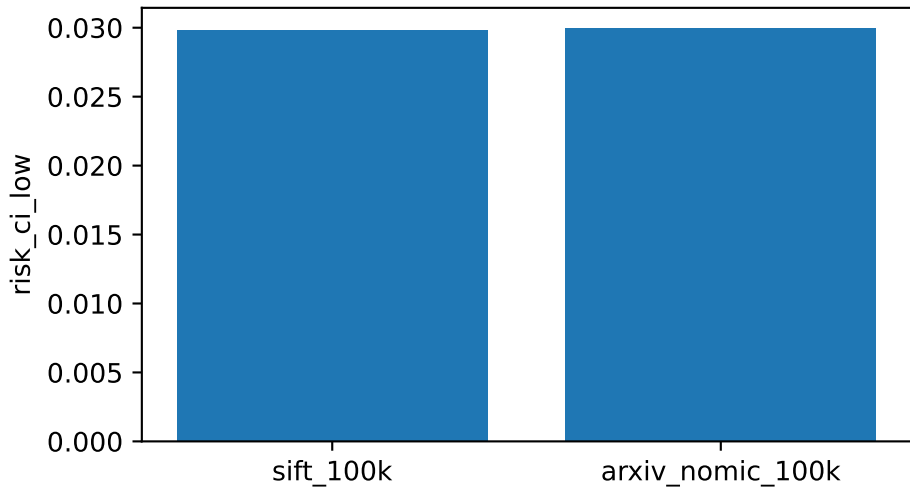
Risk CI lower bound
