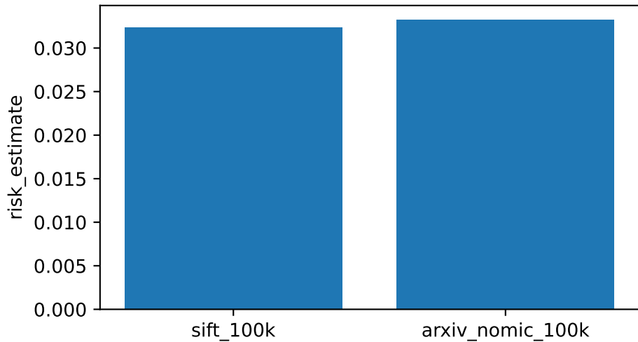
Mean-tail tradeoff
