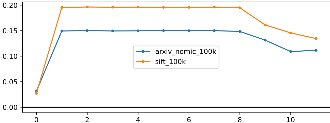
Random-only and leave-one robustness
