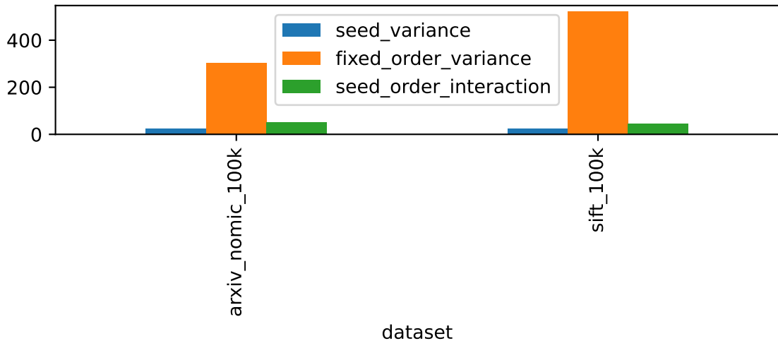
Seed and fixed-order decomposition
