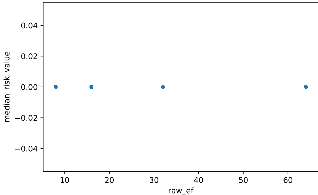
risk value
