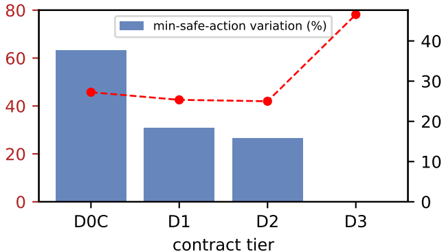
Arxiv-Nomic-100K
