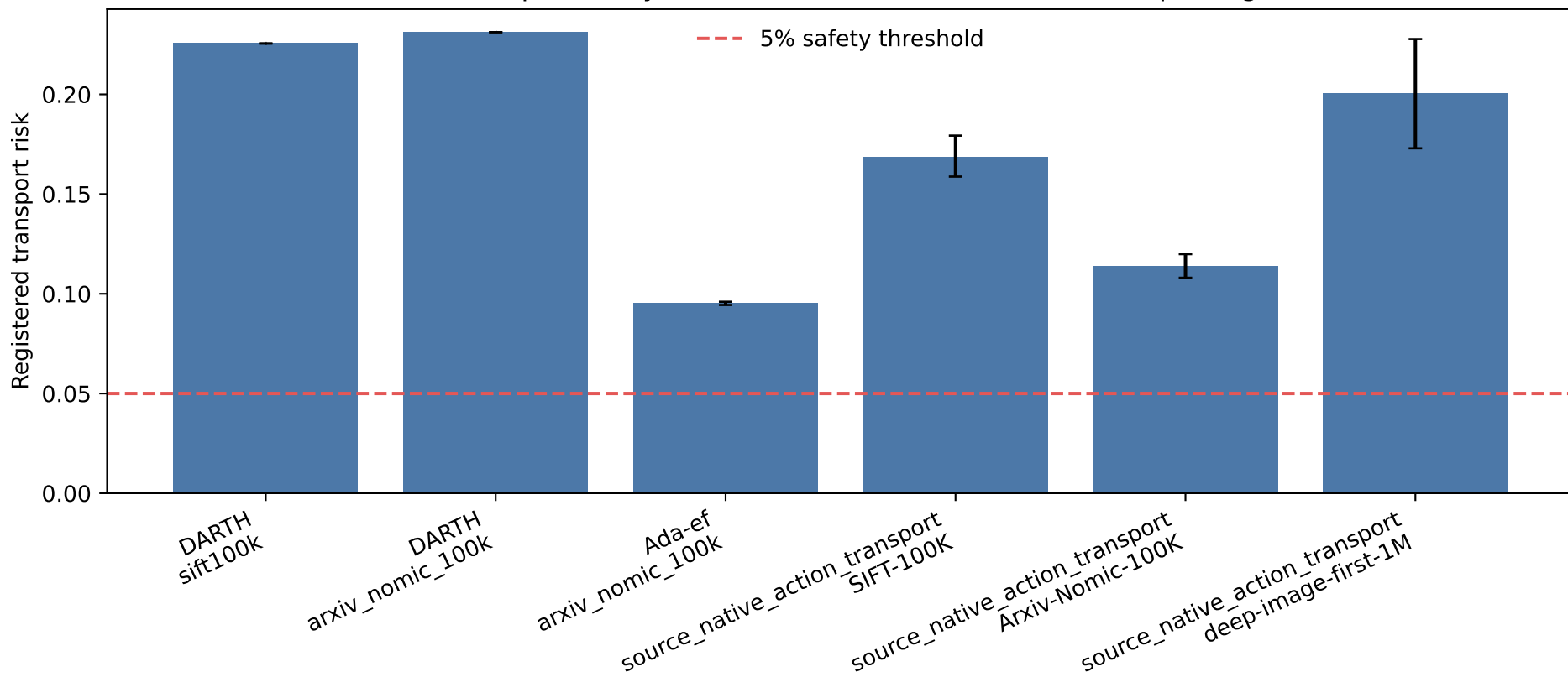
Rebuild portability evidence (stratified; no cross-action pooling)
