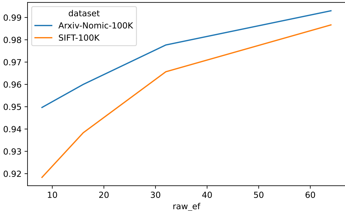
union_mean_recall
