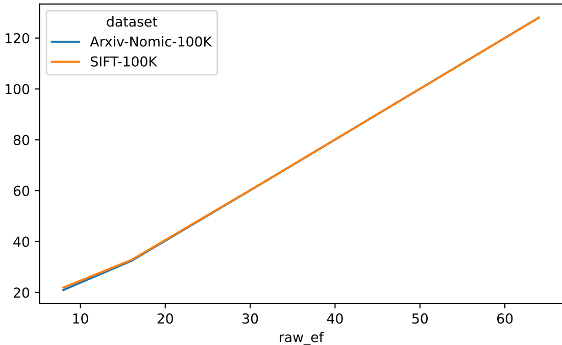
union_mean_ndc
