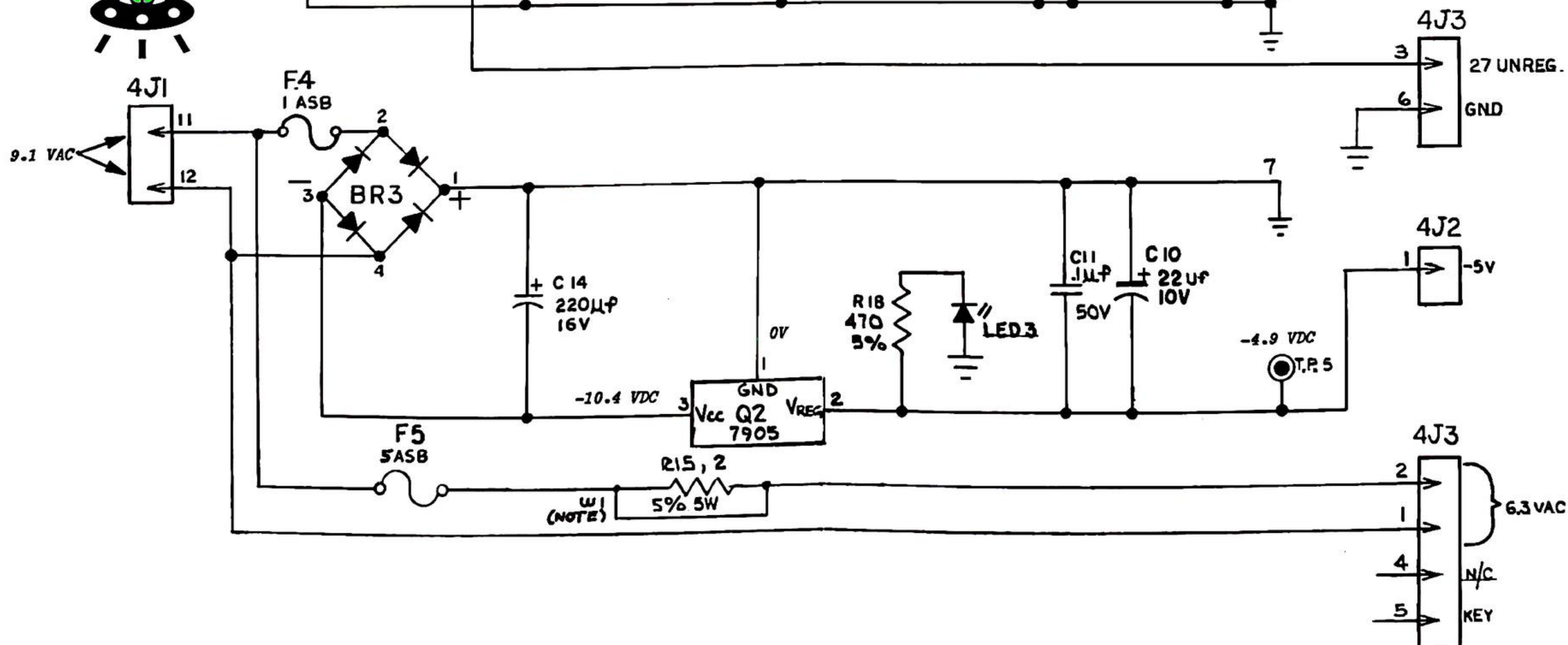
D8359 Power Supply Board Schematic Diagram
