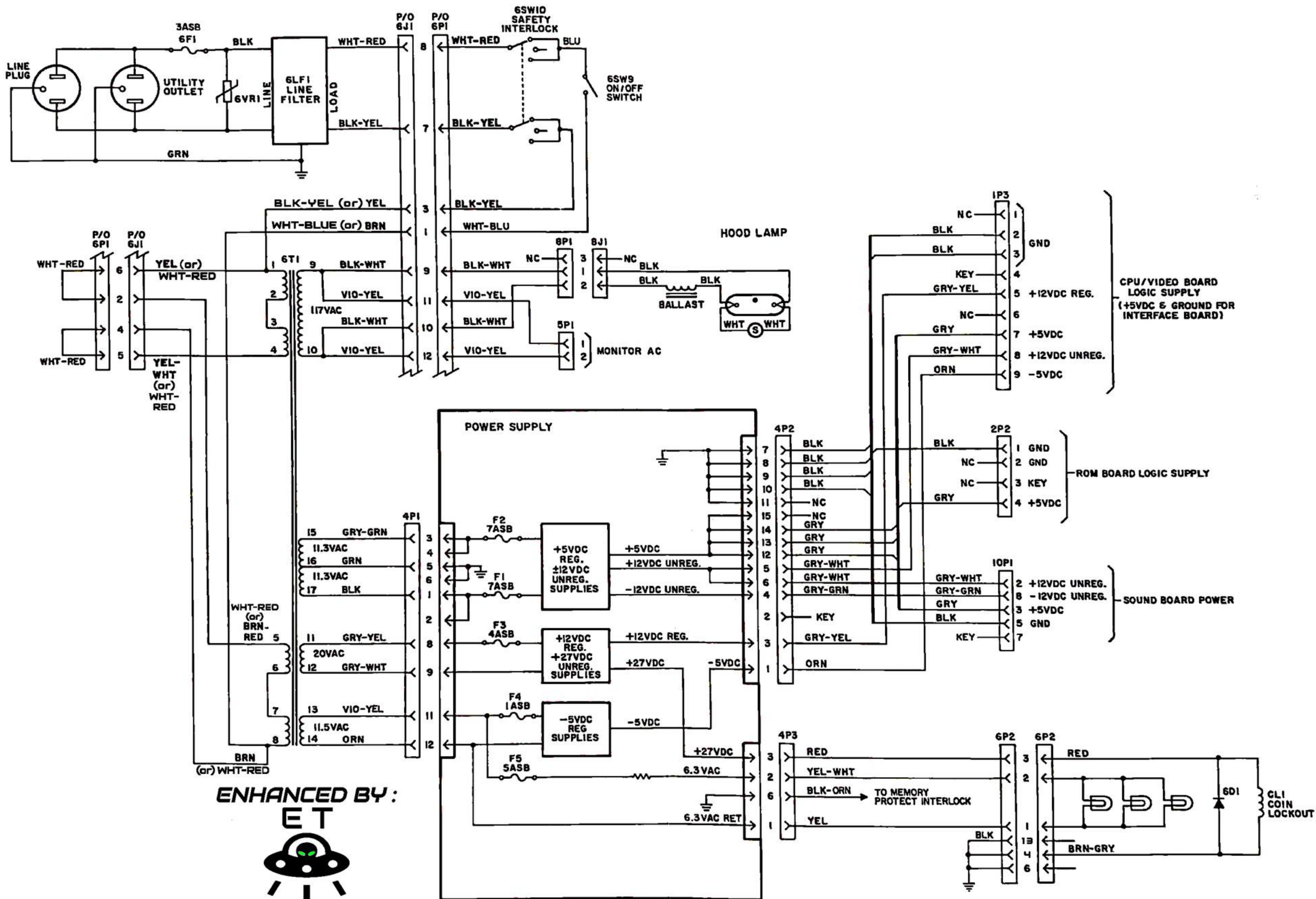
Power Wiring Diagram
