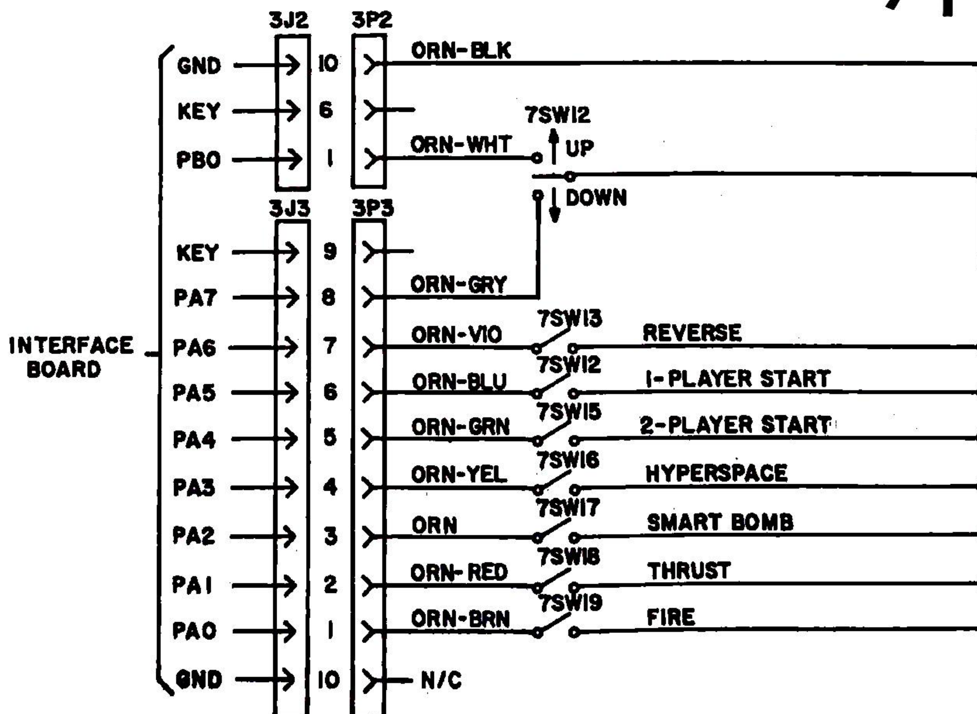
Cabinet Wiring Diagram
