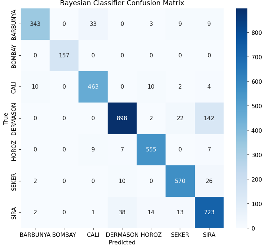
Figure 5: Bayesian confusion matrix
