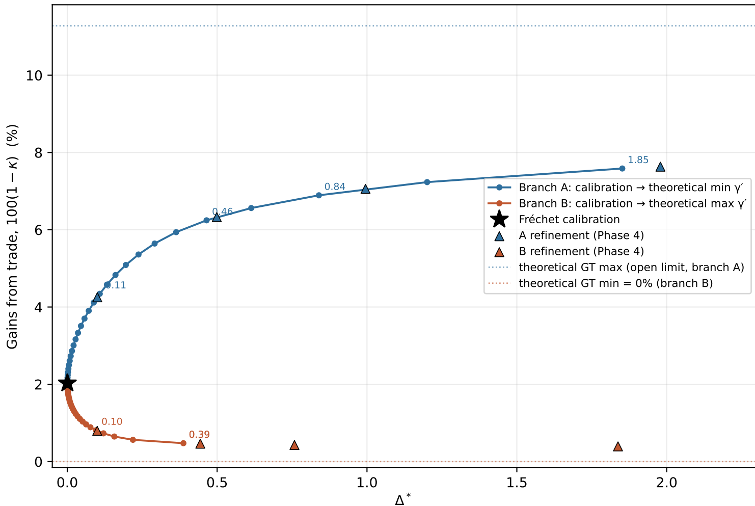
Real D=20 fixed-A/f gamma profile: gains from trade vs. \Delta^* (economically relevant region)
