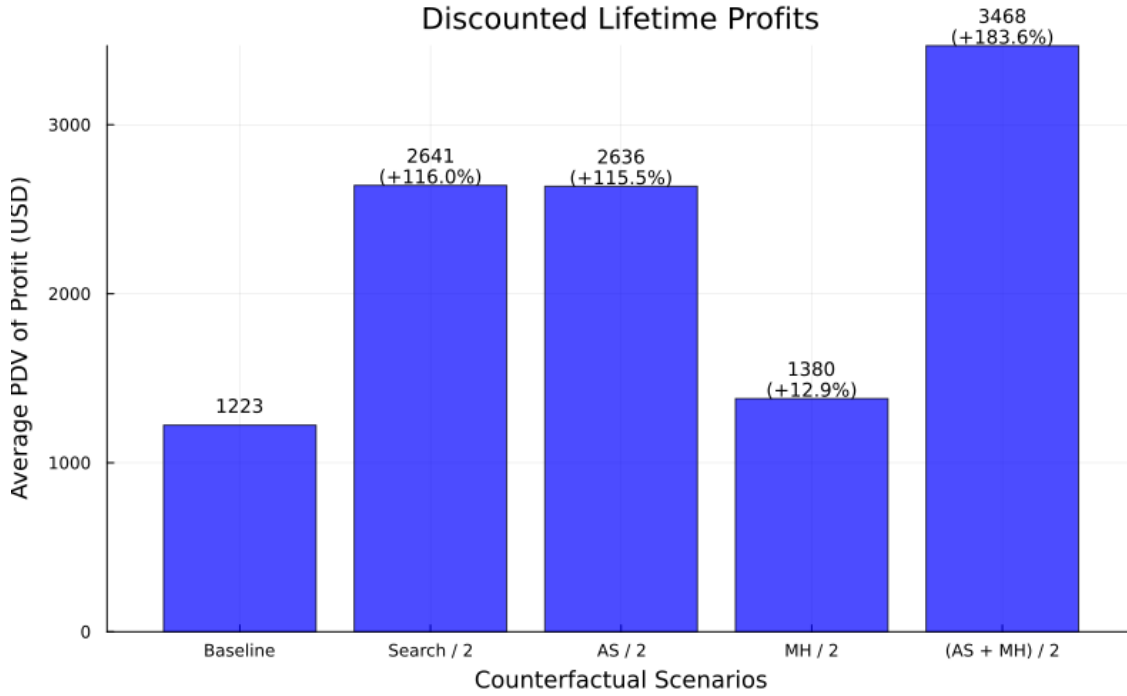
Figure 8: Counterfactuals
