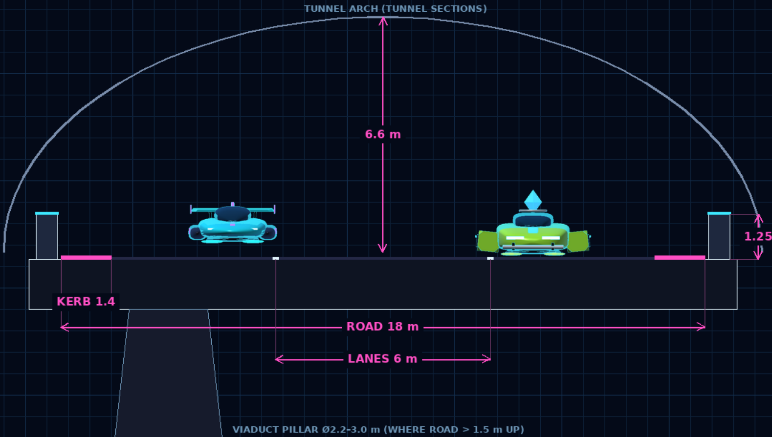
SECTION A-A · LOOKING ALONG THE RACING DIRECTION
