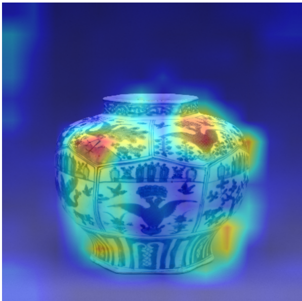
Score-CAM
