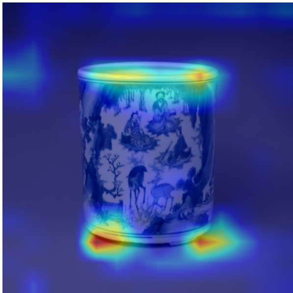
Ablation-CAM
