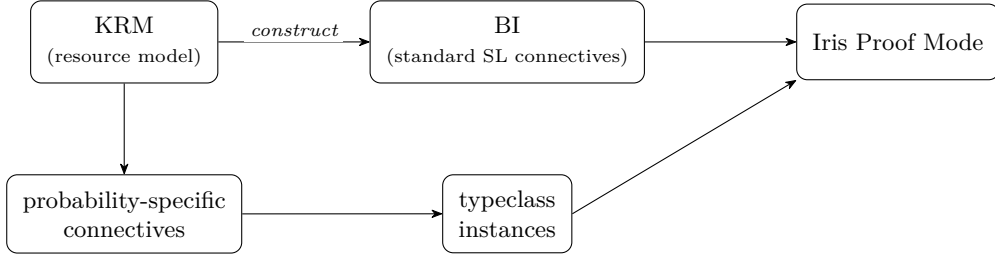
Figure 2.7: The layers of abstraction an instantiator of Iris works through. A resource model (a KRM) yields a BI by a predetermined construction, giving the proof mode the connectives and properties common to all separation logics. The connectives specific to the object logic are then defined and their characteristics registered with Iris as typeclass instances.
