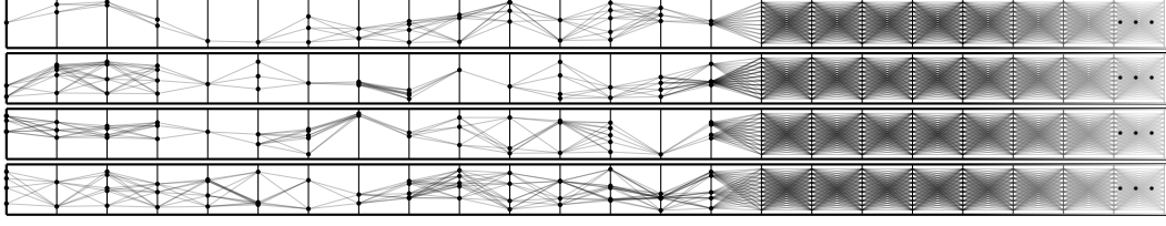
Figure 4.4: A suggestion for visualising a Finite footprint measurable space over a hilbert cube. The entire diagram is a single measurable space. Each strip makes up the measurable sets (or events) in the space. Each line in represents an infinite tuple of reals in the unit interval, connecting dots which single reals, on a vertical number line. Note that beyond the finite footprint, the lines get dense. In a fully faithful diagram, that part would be entirely filled in.
