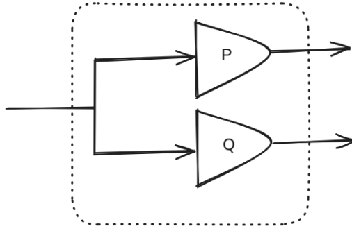
Figure 3.1: Kernel product between kernels P and Q
