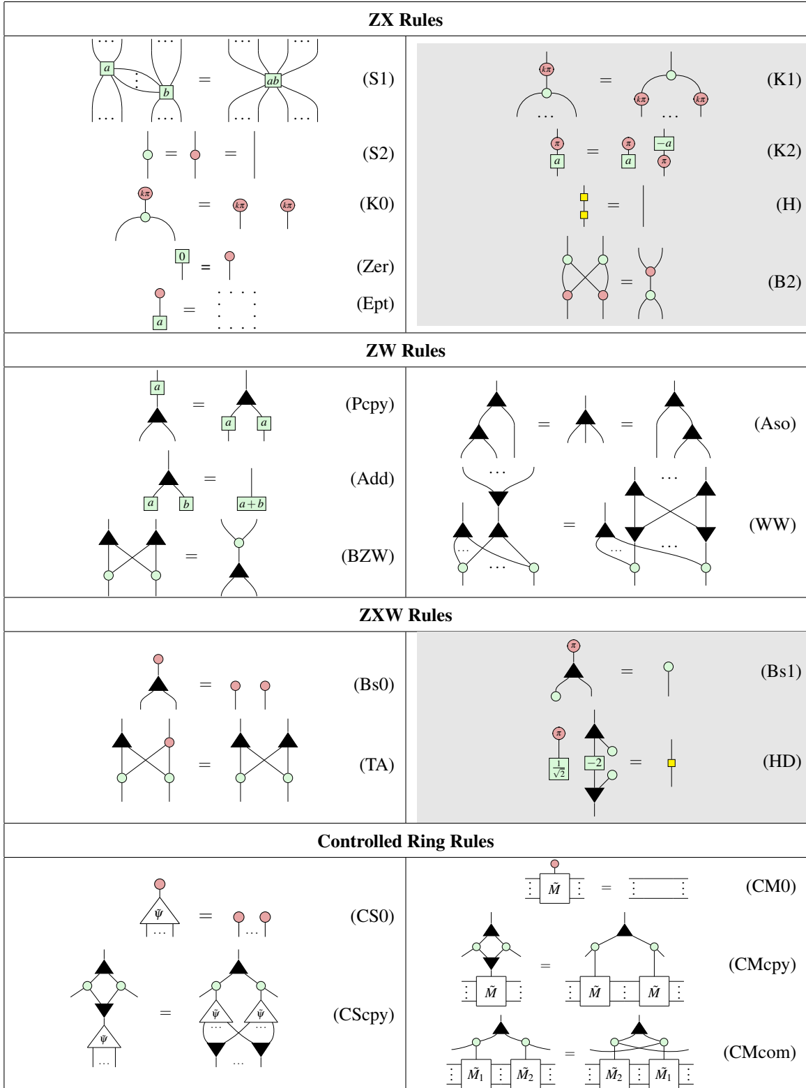
Figure 1: These ZX, ZW, and ZXW Rules are altogether complete for qubit linear maps [?], where k \in \{0, 1\} and a \in \mathbb{C} . The white background ZX, ZW, and ZXW Rules here suffice for completeness of arithmetic diagrams (Definition ??), where (??) was used only to prove Lemma ?? and we did not use the X spider case of (??). Equivalently, these complete rules for arithmetic diagrams can all be derived from the minimal qubit ZW-calculus of [?]. Adding to these the ??, ??, and ?? rules, we can show that controlled states and controlled operators form rings, culminating in Theorem ?? achieving completeness and minimality for all operations over these rings. We did not use the gray background rules in this work.
