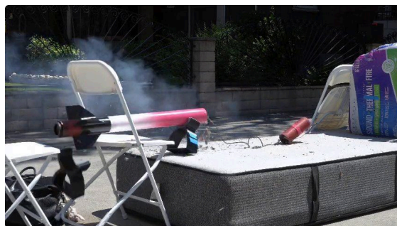
Three tenths of a second later. The booster section is coming down onto the mattress with the shock cord still attached. Frame from Bruce Duong's video.
