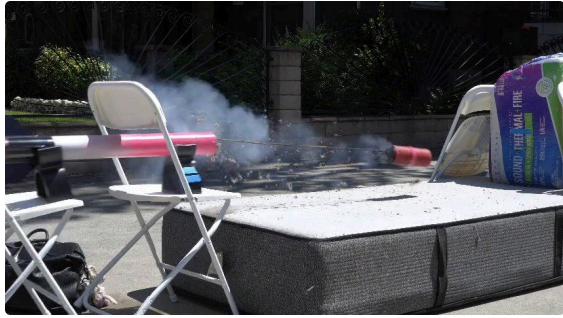
The booster ejection charge firing during the two-stage pop test on MTD3, 30 August 2026. The coupler is already out of the tube and the shock cord is taut. Frame from Bruce Duong's video of the test.
