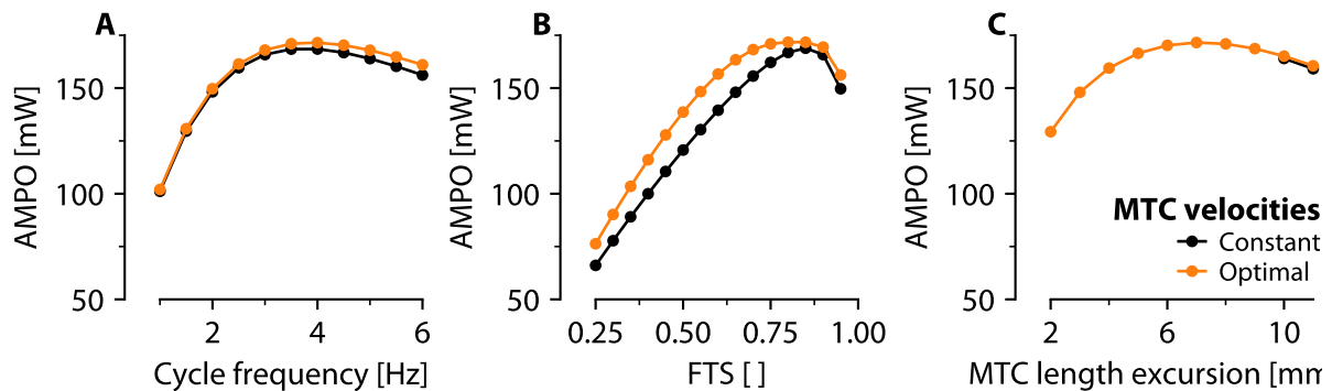
Figure S3.2: Predicted influence of cycle frequency (A), FTS (B) and MTC length excursion (C) on the maximum attainable AMPO. The maximally attainable AMPO — averaged across the three rats — slightly increased in SSCs without a constraint on MTC length over time (orange lines), compared to SSCs with a constant MTC shortening and lengthening velocity (black lines).
