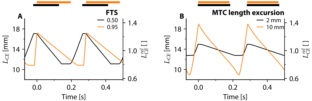
Figure S3.1: Predicted CE length over time for maximally attainable AMPO, shown for two imposed FTS values (A) and two imposed MTC length excursions (B), at a cycle frequency of 3.5 Hz for rat 1. In panel A, only cycle frequency and FTS were imposed, while in panel B only cycle frequency and MTC length excursions were imposed. Apart from these two constraints, CE and MTC length over time were completely unconstrained and thus the shape of CE length over time could be different between every combination of imposed cycle frequency and FTS (A) or imposed cycle frequency and MTC length excursion (B). CE stimulation was maximal during the period indicated by the coloured bars, and ‘off’ elsewhere.
