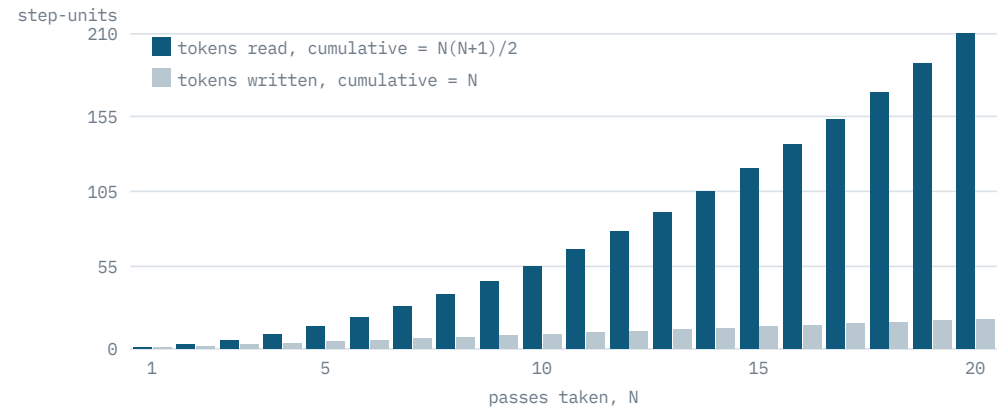
Tokens read and written over a task, in units of “tokens added per pass”, with the full history re-sent and no cache (calc.).
