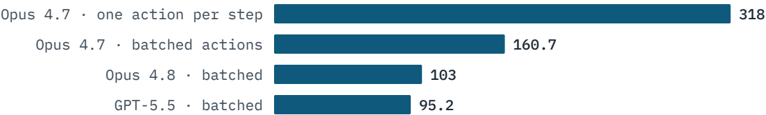
Steps per task on OSWorld 2.0, 108 tasks
