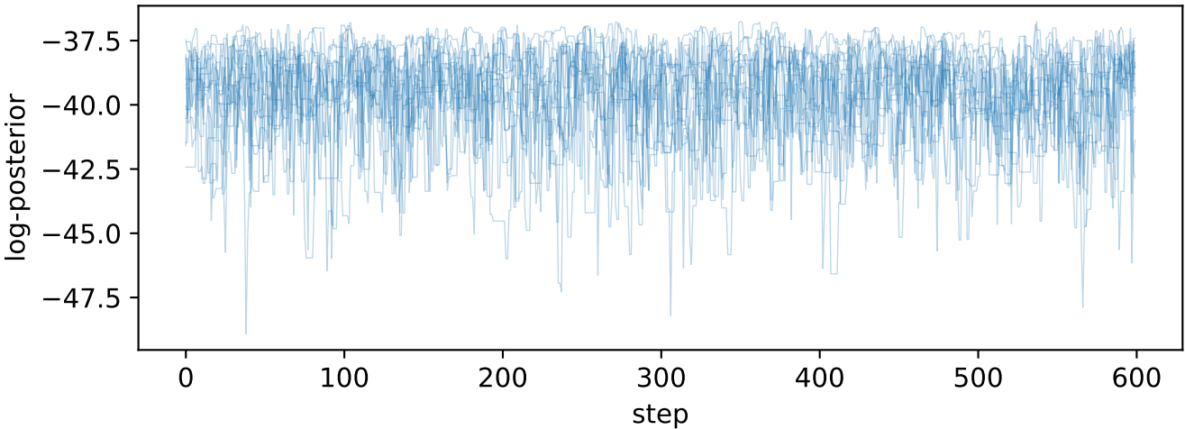
Log-posterior across walkers
