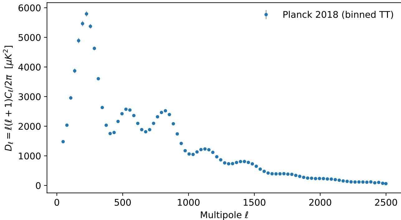
Planck 2018 binned TT power spectrum
