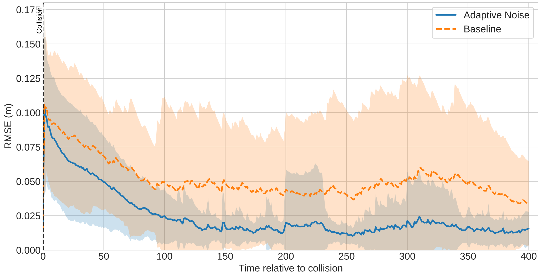
Collision-Aligned RMSE: Baseline vs Adaptive Noise
