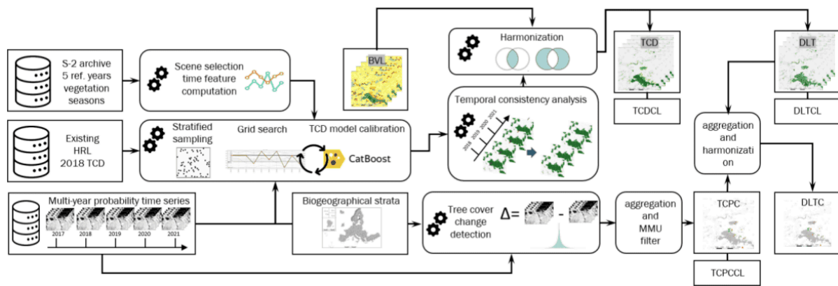
Figure 3: High-level flow chart of the production workflow for the Tree Cover & Forests products TCD, DLT, TCPC and DLTC.
