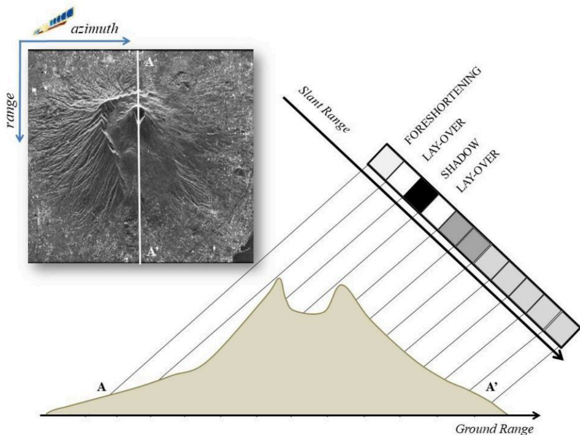
Figure 7: SAR amplitude image acquired over the Vesuvius volcano. Studying a range line passing through the caldera (section A-A') shows pixels affected by foreshortening, layover, and shadowing, as well as areas characterised by good spatial sampling (although with low reflectivity values) along the slopes facing away from the sensor (adapted from Ferretti, 2014).
