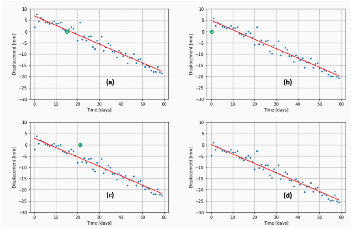
Figure 26 Temporal reference point. (a) The time series is referred to the primary image (circled in green). (b) The time series is referred to the first image in the dataset (circled in green). (c) The time series is referred to a particular noisy image (circled in green). (d) The time series is referred to the origin of the fitted model (the red line).
