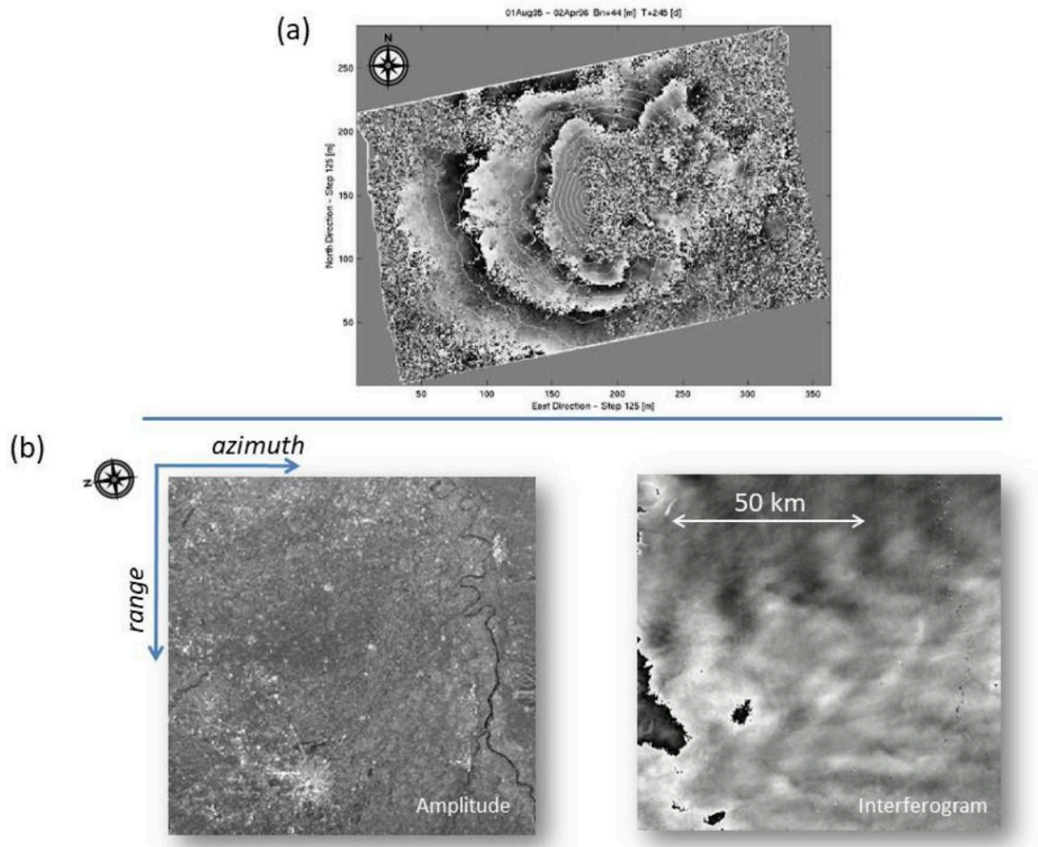
Figure 25 (a) Example of propagation anomalies generated by atmospheric stratification. The area of interest is the Etna volcano in Sicily. Interferometric fringes resemble the contour lines of the volcano. (b) Amplitude data and differential interferogram over the Po valley in Italy. Fringes are generated by tropospheric effects.
