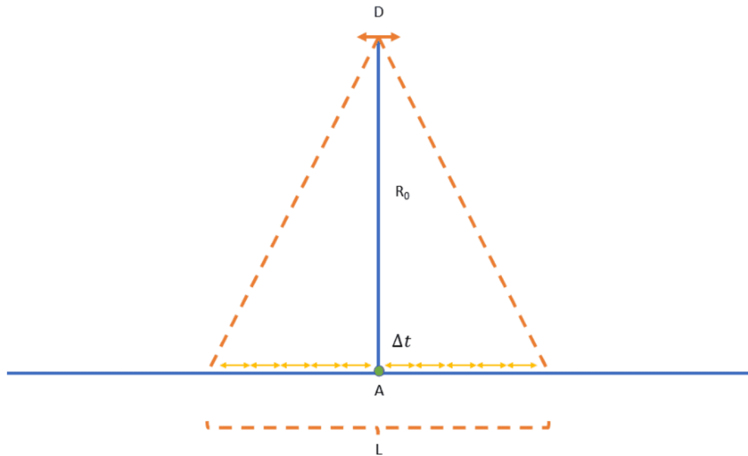
Figure 4 Synthetic Aperture geometric representation.
