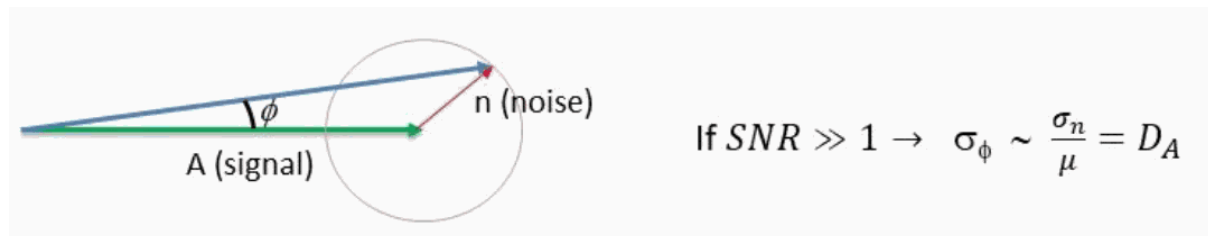
Figure 19 Model behind the use of the amplitude dispersion index (DA) as a proxy for phase stability. The complex noise is supposed to be circular and Gaussian having the same standard deviation \sigma_n for both the real and the imaginary component. \mu represents the incoherent average of all the signal vectors A . If the signal-to-noise ratio is well above the value of 1, the ratio between \sigma_n and \mu is a good estimator of the phase dispersion \sigma_\phi .
