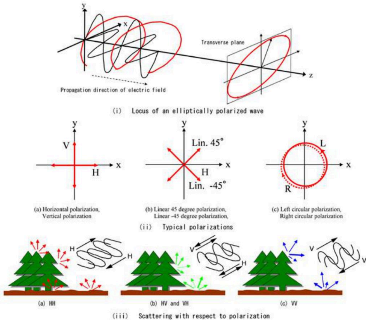
Figure 6 Example of electromagnetic wave polarization applied to remote sensing. From https://www.eorc.jaxa.jp/ALOS/en/img_up/pal_polarization.htm
