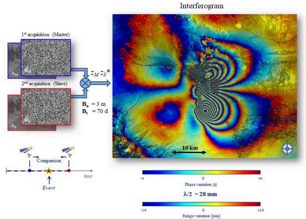
Figure 9 Formation of an interferogram.
