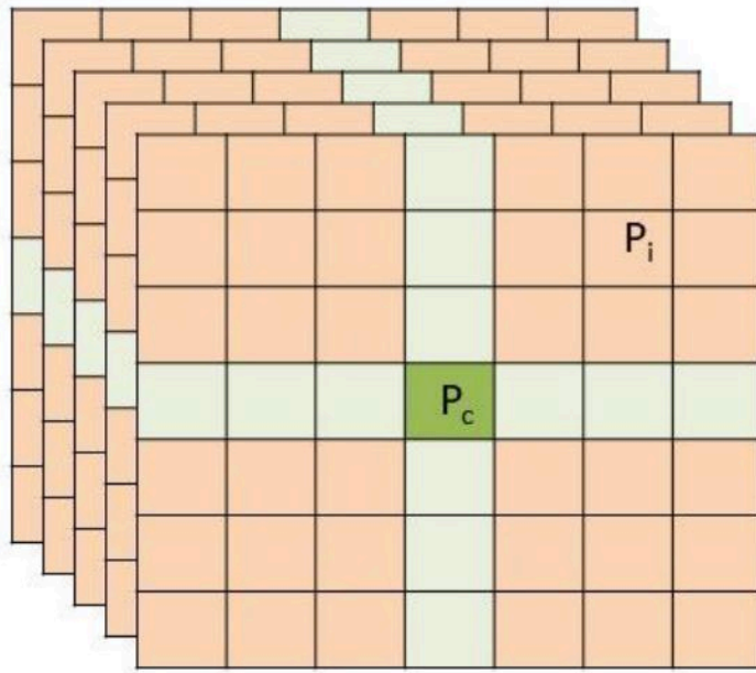
Figure 20 Computation of the signal-to-clutter ratio (SCR). A is the amplitude of the radar image. P_c is the pixel under analysis and P_i is the generic pixel of the “red areas” where the clutter power is estimated. Green pixels are considered heavily impacted by sidelobes of P_c . Working on a SAR datastack, the SCR is computed for each image first and results are then averaged.
