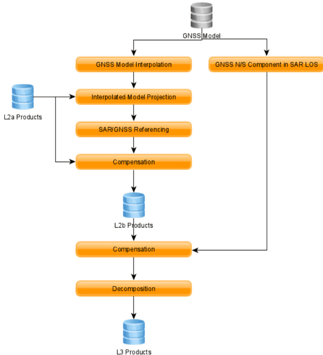
Figure 36 L2b products calibration process.
