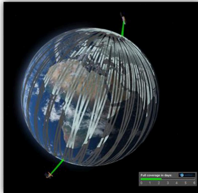
Figure 30 Sentinel-1 constellation acquisition by relative orbit. https://sentinels.copernicus.eu/web/sentinel/missions/sentinel-1/satellite-description/orbit
