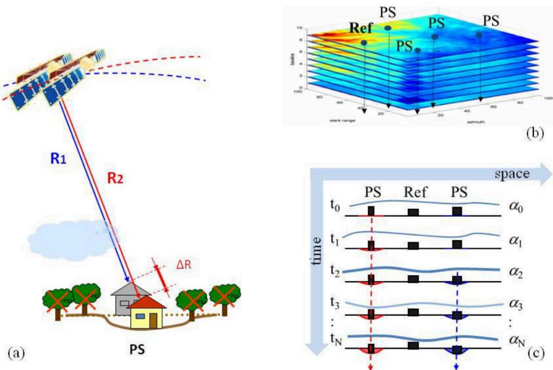
Figure 11: a) multi-interferogram techniques aim at identifying coherent radar targets (referred to as persistent scatterers) that are only slightly affected by phase decorrelation. b) Given a data stack of multi-temporal SAR acquisitions, the analysis is carried out on a sparse PS grid, rather than on all image pixels. c) After PS identification and reference point selection, atmospheric effects are estimated and removed taking advantage of their statistical behaviour. The APS superimposed on each SAR image is almost uncorrelated in time, but is correlated spatially, while displacement phase components are usually correlated in time. (Adapted from Ferretti, 2014).
