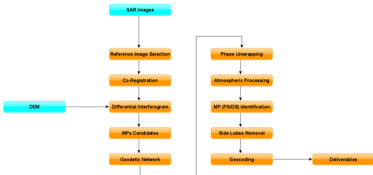
Figure 13 Representation of a generic InSAR processing chain.
