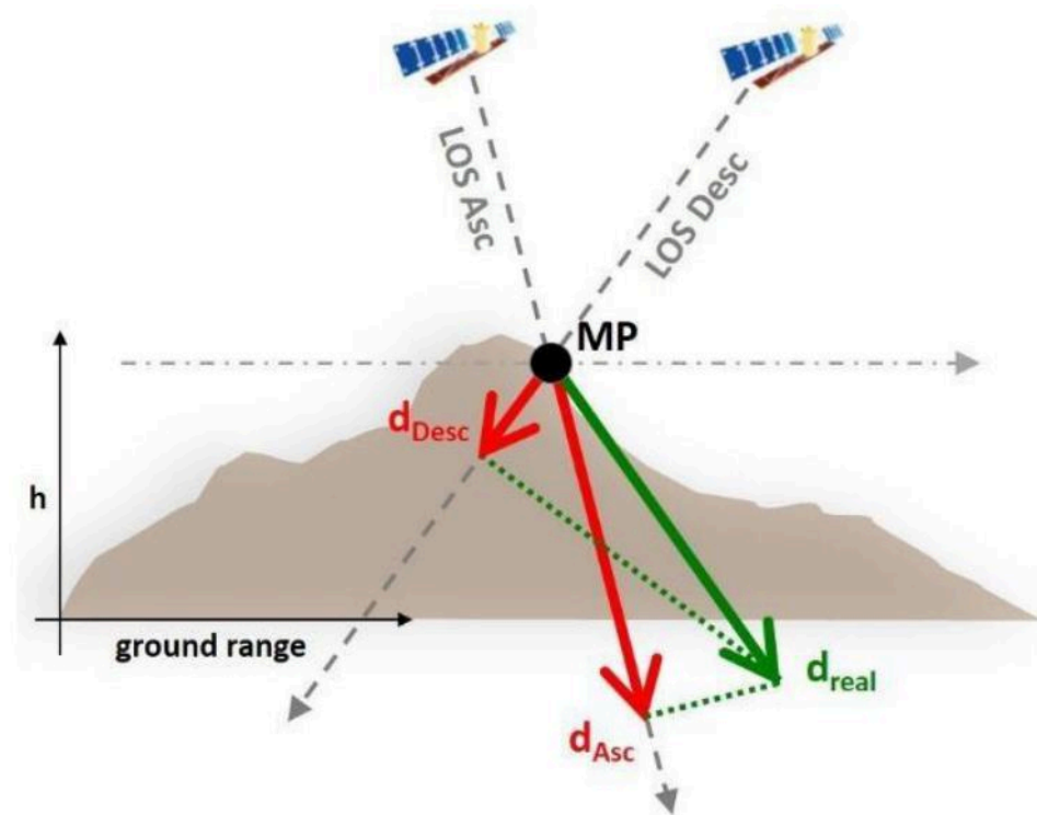
Figure 37 The same real displacement can result in different measured displacements if viewed from different angles.
