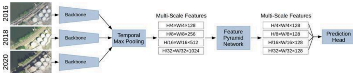
Model architecture of SATLASNET. Separate heads can be used to predict outputs of different formats or different thematic nature (source: Bastani et al, 2023)
