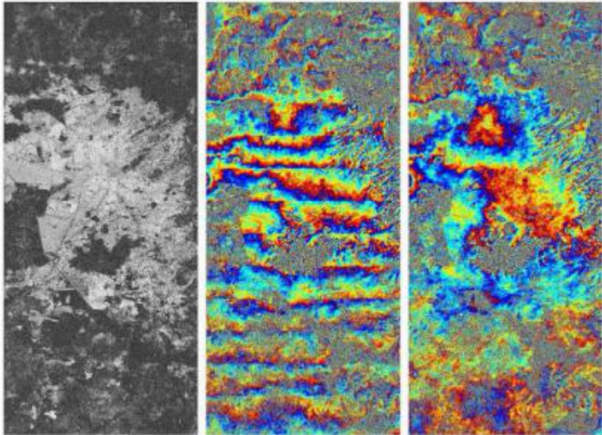
Figure 16 - Prats et al., 2012 - Example of along-track linear phase ramps in a TOPS interferogram due to an artificially induced azimuth constant registration error (middle). Interferogram coherence (left). The same interferogram without azimuth registration error (right).
