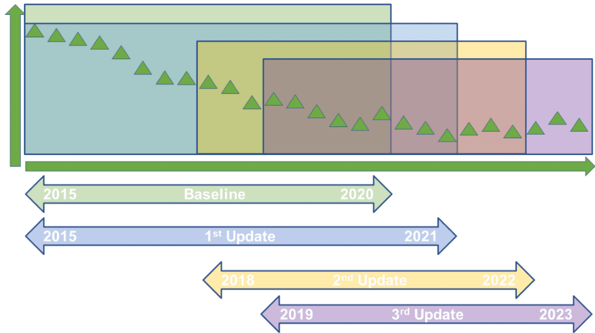
Figure 44 L2a data. Future updates policy. A 5-year sliding window is used to select the data.
