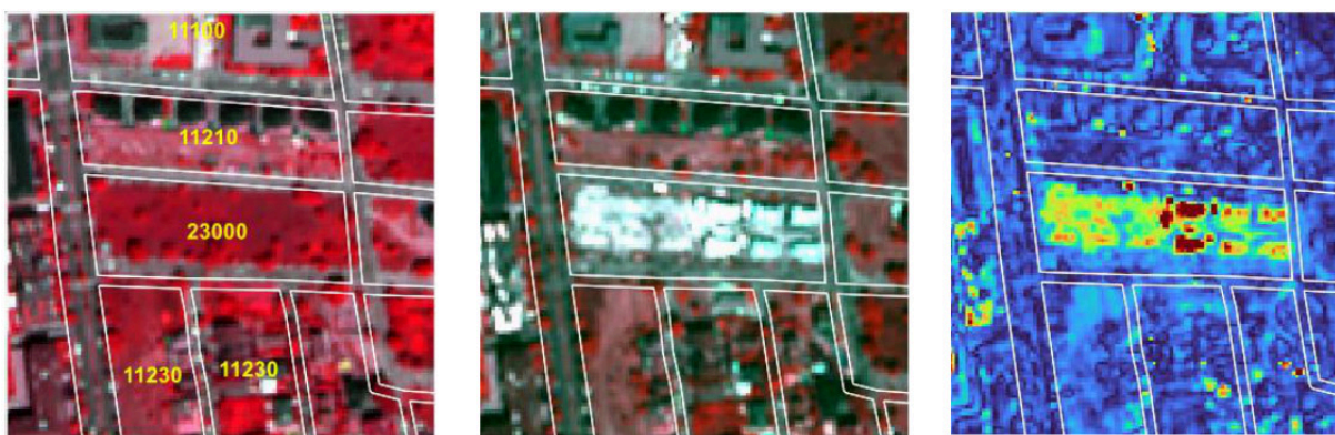
Change detection heatmap derived from VHR data (left: VHR2018 and UA2018 product; centre: VHR2021; right: Change heatmap where changes are highlighted in yellow/red) (location: Madrid, Spain)
