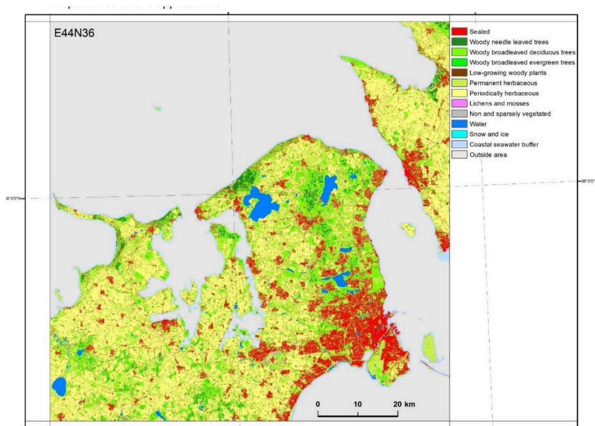
CLCplus Backbone 2023 for tile E44N36 (Copenhagen)
