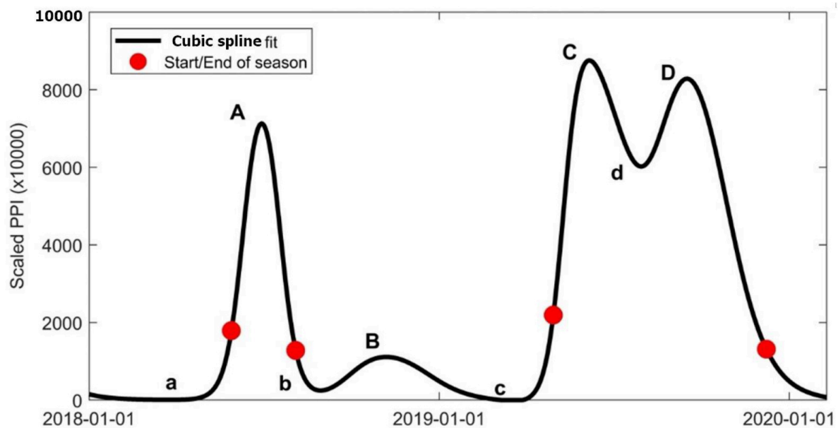
Figure 6. Illustration of season identification based on coarse-season peaks (A-D) and corresponding local minima (a-d). Red markers indicate season start and end points.
