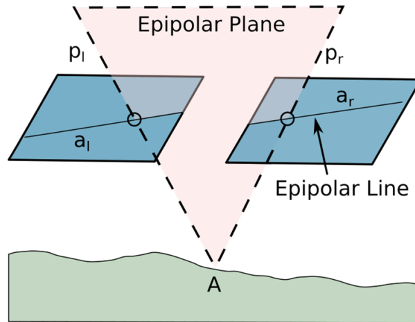
Figure 6-9 Schematic representation of the epipolar geometry for a given pair of satellite images, on which the AI-EOSURFACE algorithm is based to obtain elevations
