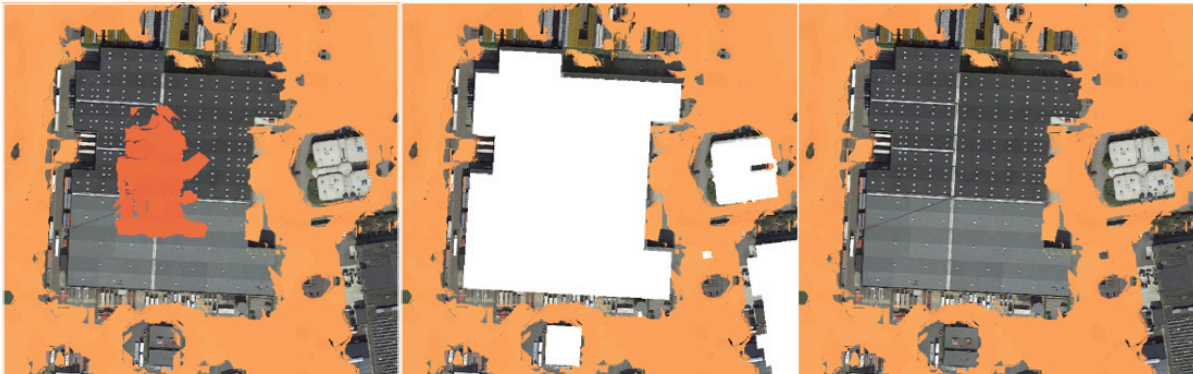
Figure 6-10 DSM filtering to remove large buildings and obtain the DTM
