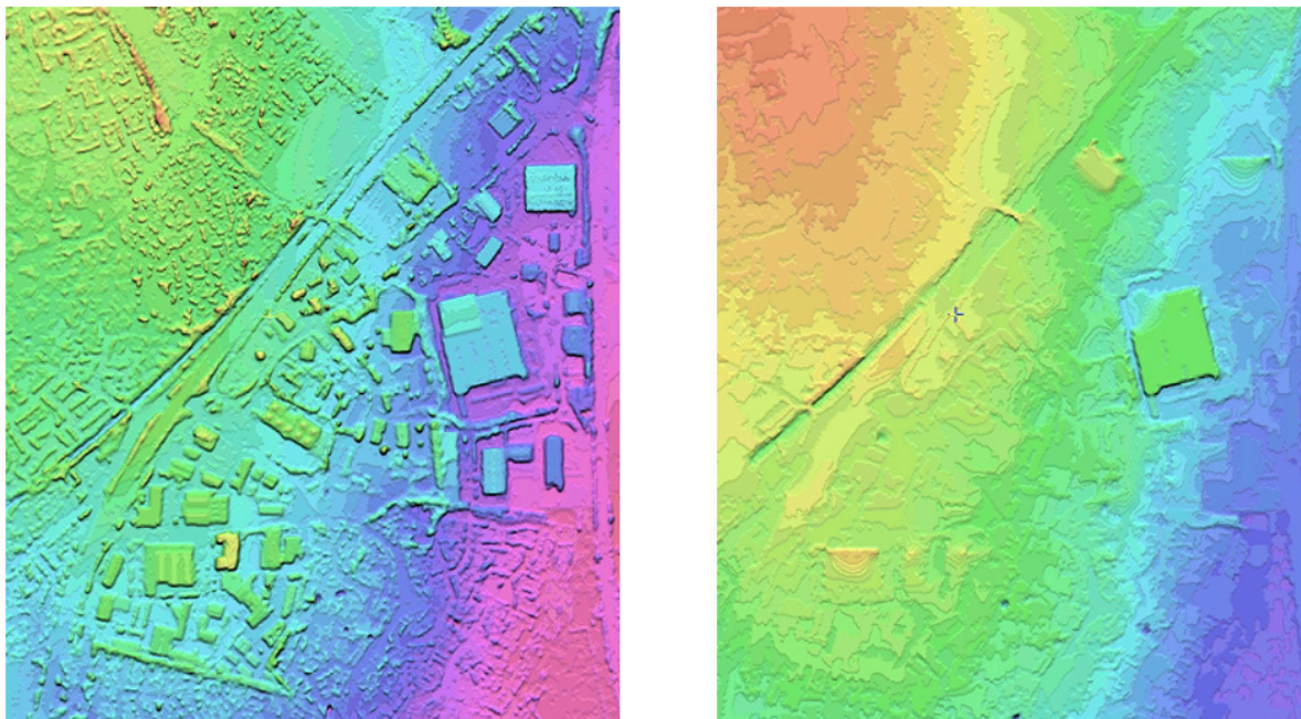
Figure 6-11 Left: DSM for an area in London. Right: DTM for an area in London
