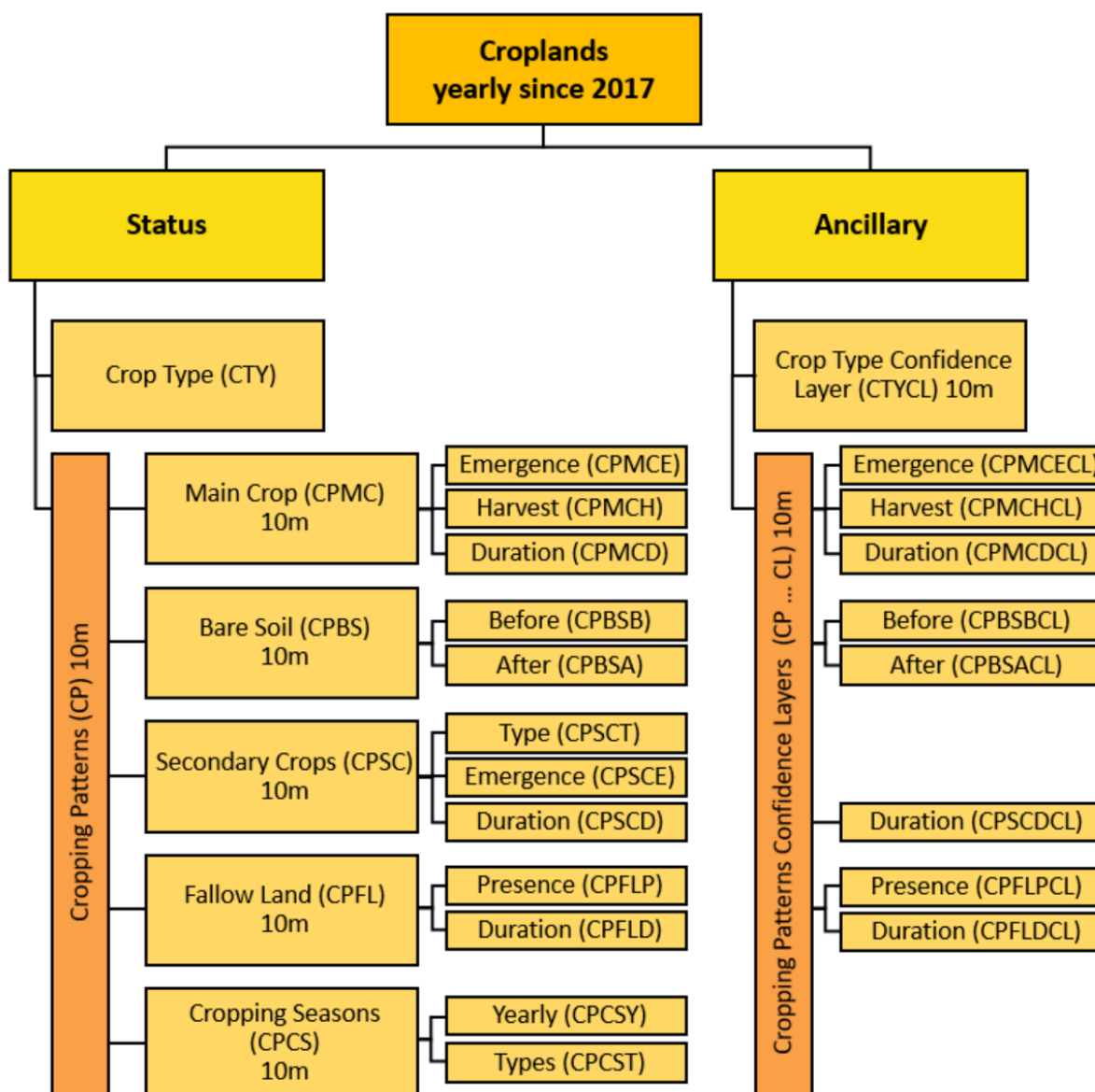
Figure 7-2 HRL Croplands product overview
