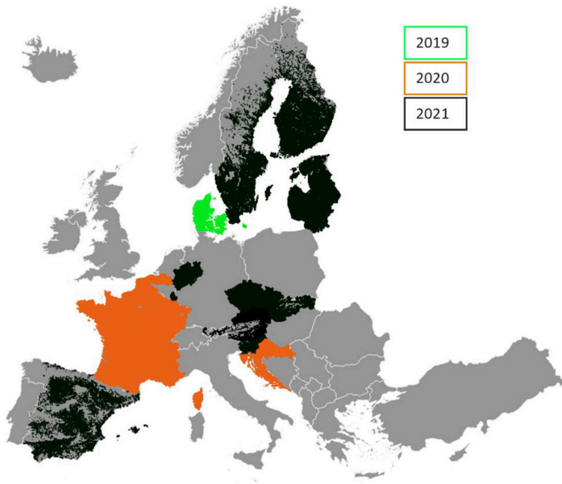
Figure 8-4: GSAA data availability, per country per year
