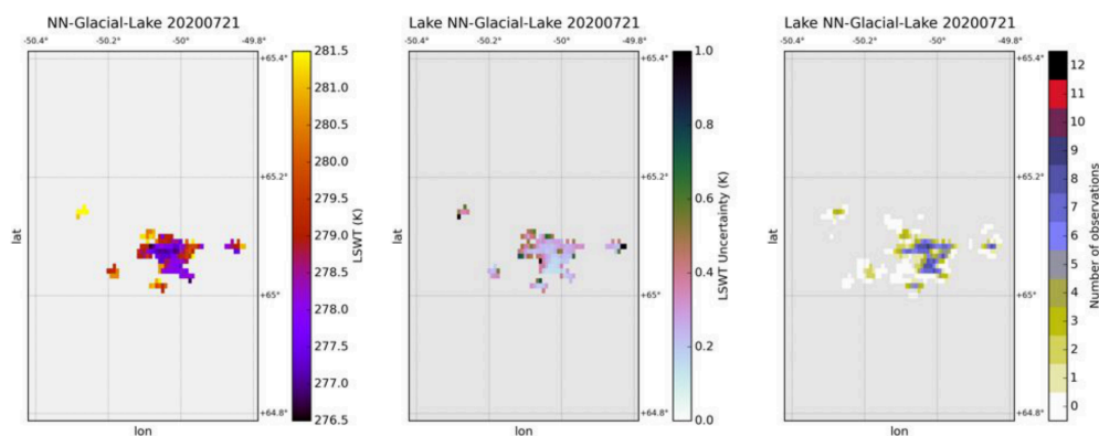
Figure 4: LSWT, uncertainty and number of observations for a glacial lake in Greenland (centre lat=65.087, lon=-50.040, maximum distance from land = 1.8 km) for the 10-day period starting on the 21-Jul-2020 using SLSTR-AB data.
