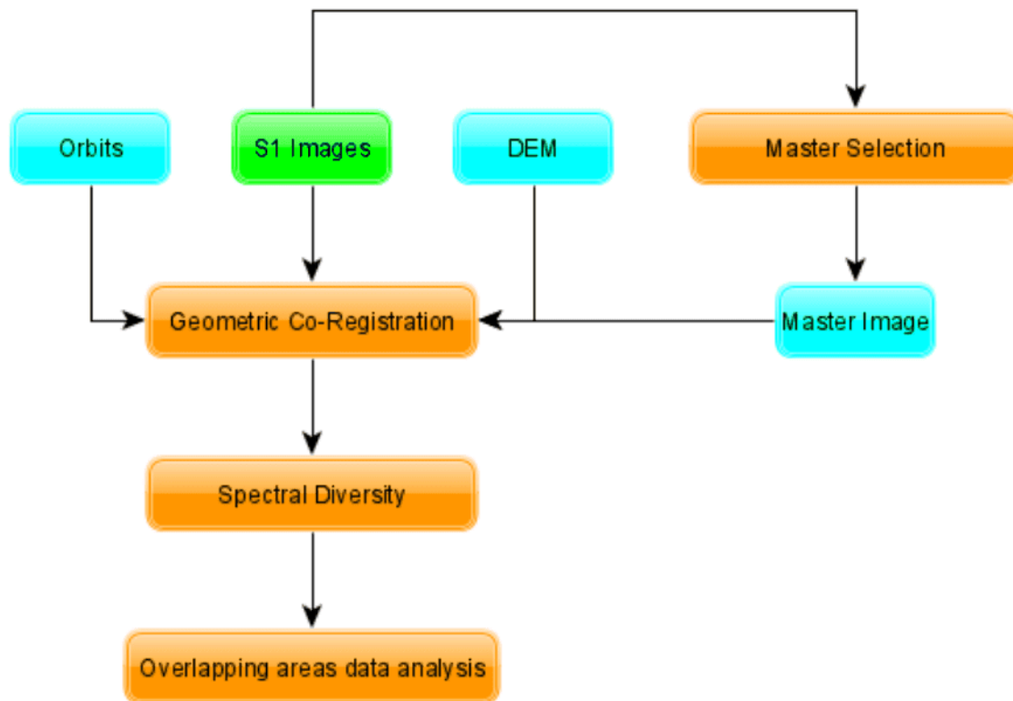
Figure 15 Co-registration workflow.
