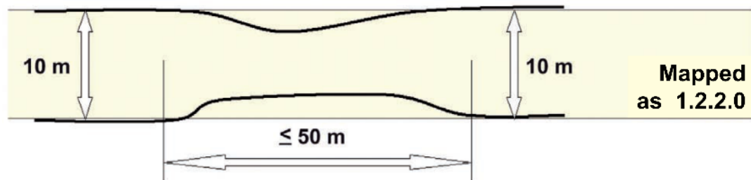
Figure 11: MMW exception
