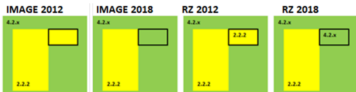
Figure 18: Simple change
