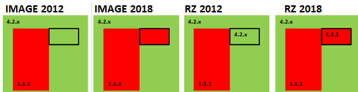
Figure 17: Simple change
