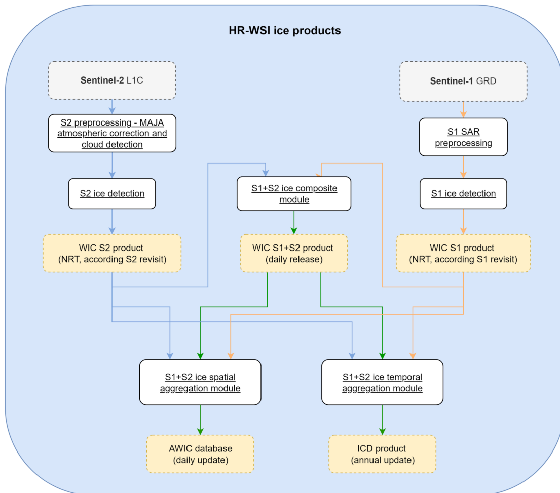
Figure 1. HR-WSI ice production workflow (NRT: near real-time). The colored arrows distinguish the processing of data derived from Sentinel-1 (orange), Sentinel-2 (blue) and both Sentinel-1 and Sentinel-2 (green) acquisitions.
