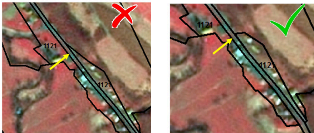
Figure 7: Delineation avoiding acute angles
