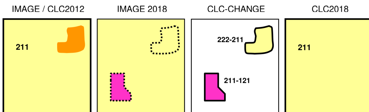
(222) > 5 ha disappears because of being turned into arable land (211). Both patches must be delineated as changes (211-121 and 222-211), as being > 5 ha. No new polygons emerge in CLC2018, as corresponding change polygons are generalised.
