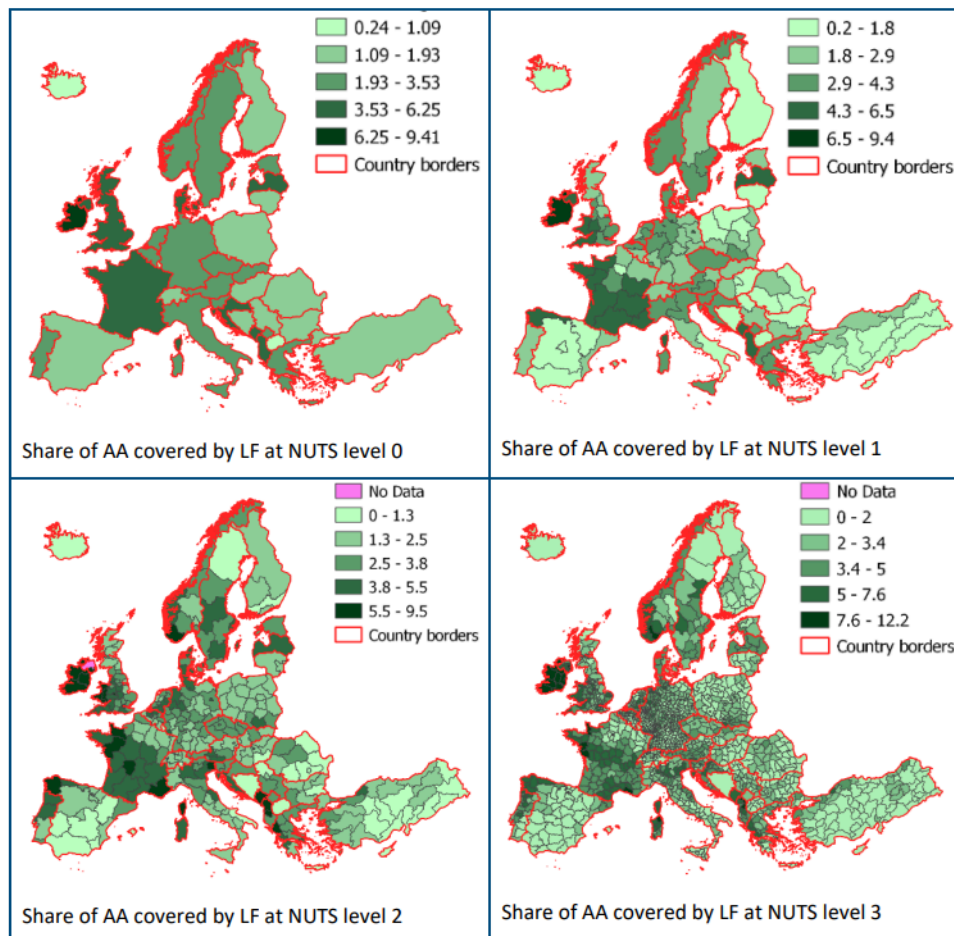
Figure 1: Share of agricultural area (AA) covered with woody landscape features at different NUTS levels based on SWF 2015
