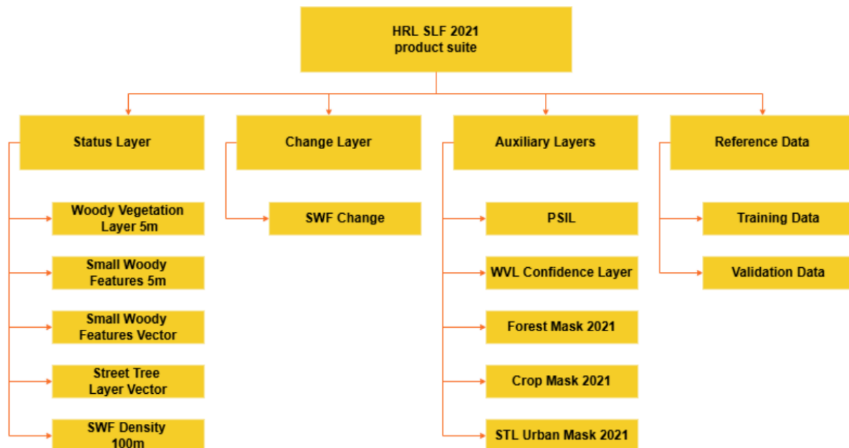
Figure 2: HRL SLF 2021 product suite
