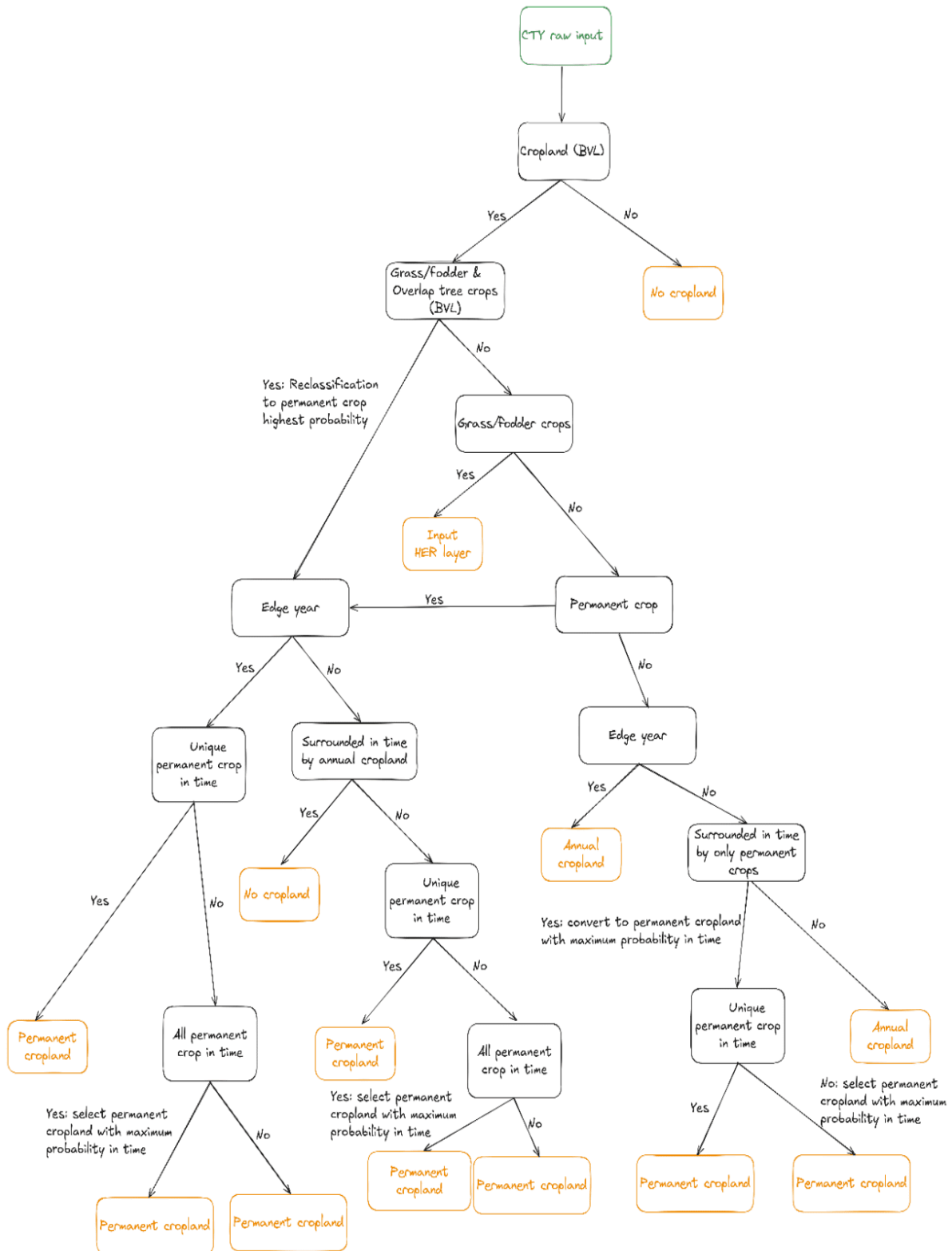
Figure 20: Figure 20: Decision tree of the CTY postprocessing pipeline, outlining the main steps from raw crop type probabilities to final output classes. For clarity, output categories are simplified to 'permanent' and 'annual' cropland, as the decision rules were specifically designed for these classes. Note that spatial operations (defined in Figure 19) such as spatial smoothing and GDAL Sieve, although they may further modify crop type labels, are not included in this diagram to maintain readability
